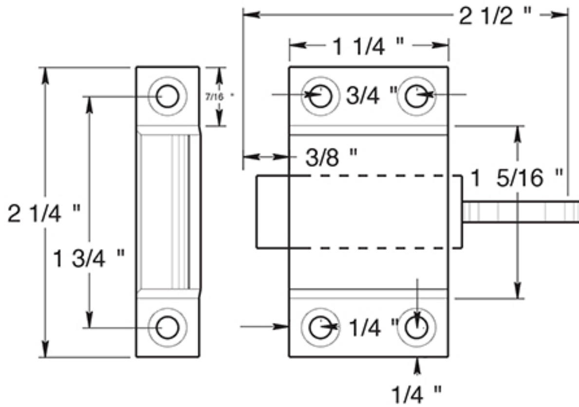
TOP VIEW
