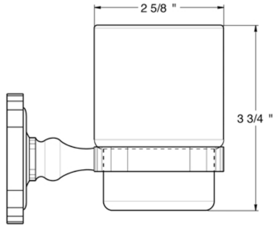
SIDE VIEW
